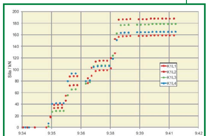
Checking of the ground anchor tensioning process
