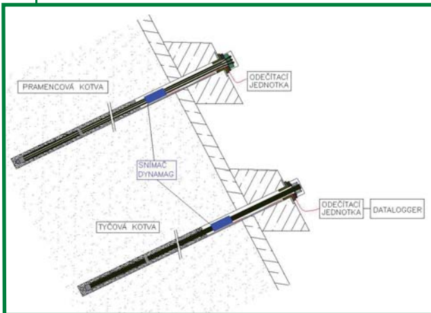
Sensors application on ground anchors
