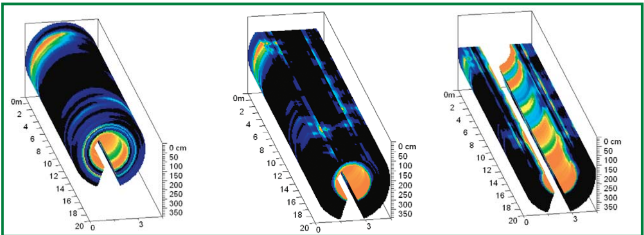
3D processing of ground-penetrating radar measurements
