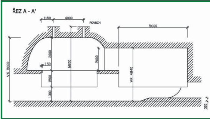
plan of chamber
