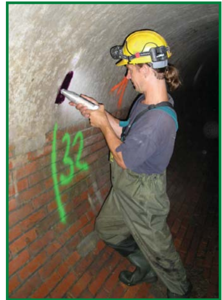
Schmidt impact hammer test
