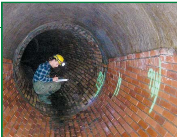
documentation of the technical state with denotation and description of fault
