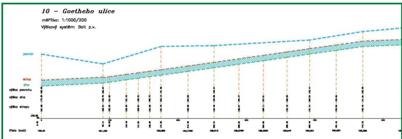
longitudinal profile of conduit measurement
